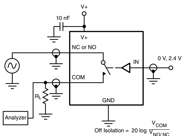
Figure 3. Off-Isolation
