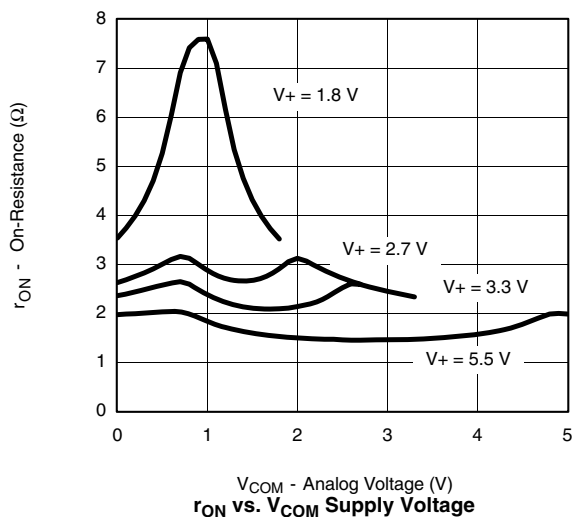
r_{ON} vs. V_{COM} Supply Voltage
