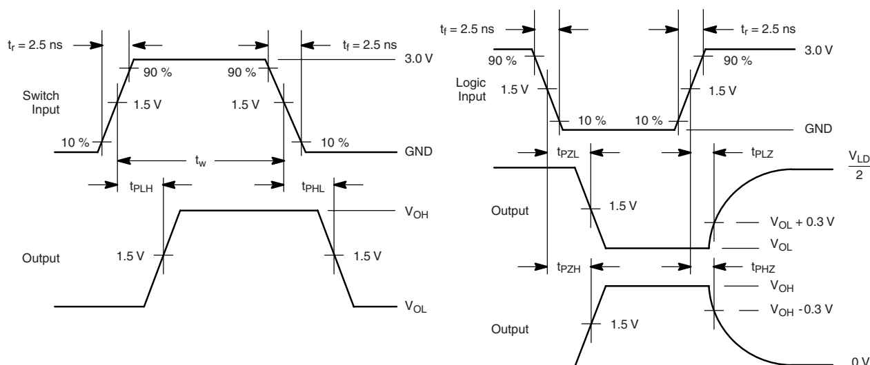
Figure 2. AC Waveforms
