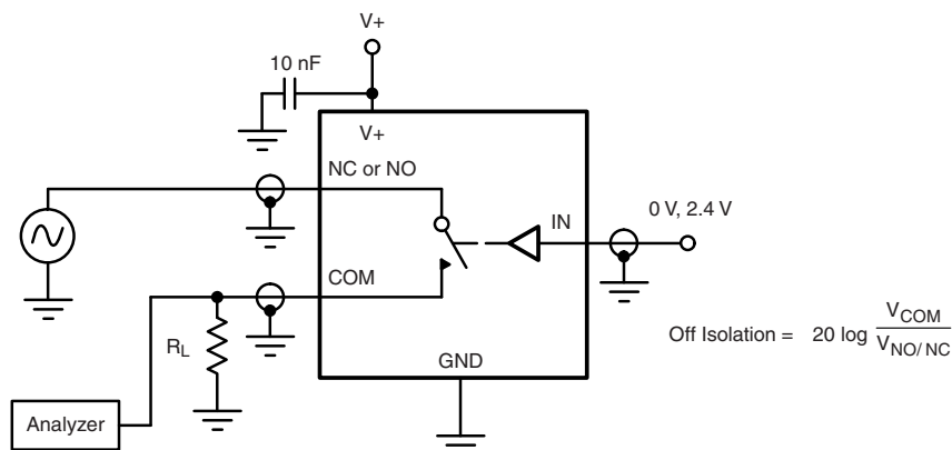
Figure 3. Off-Isolation
