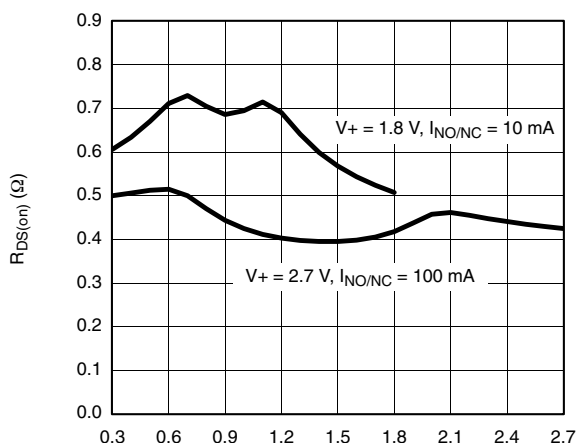
R_{DS(on)} vs. V_{COM} vs. 1 V_{CC}
