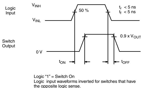
Figure 1. Switching Time
