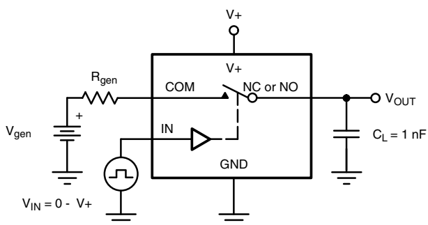
Figure 2. Charge Injection
