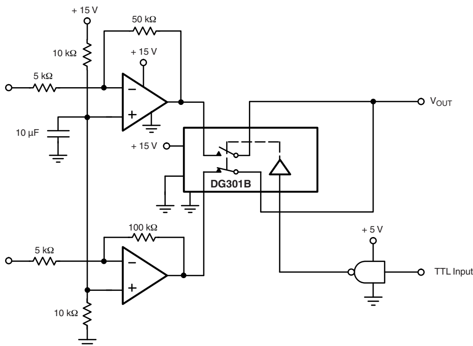
Figure 5. Single Supply Op. Amp. Switching
