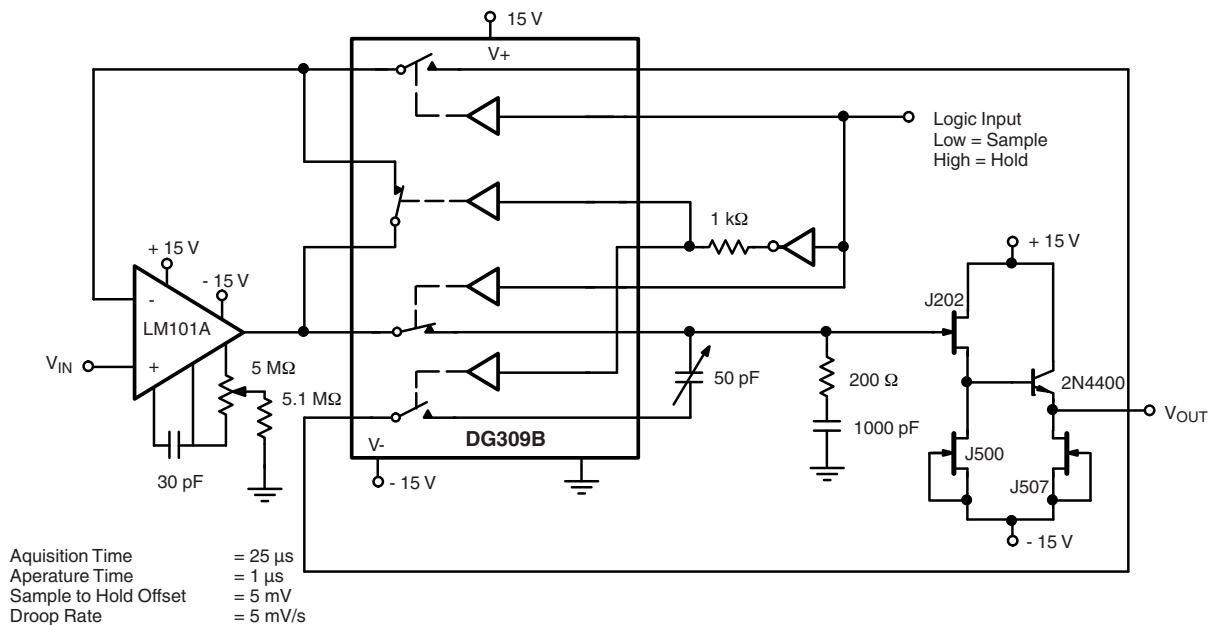
Figure 7. Sample-and-Hold
