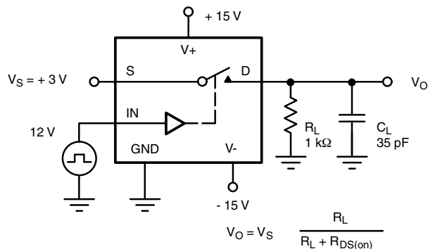
Figure 2. Switching Time
