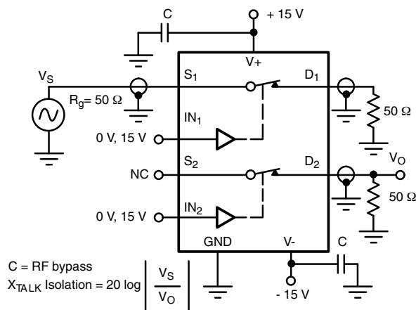
Figure 4. Channel-to-Channel Crosstalk
