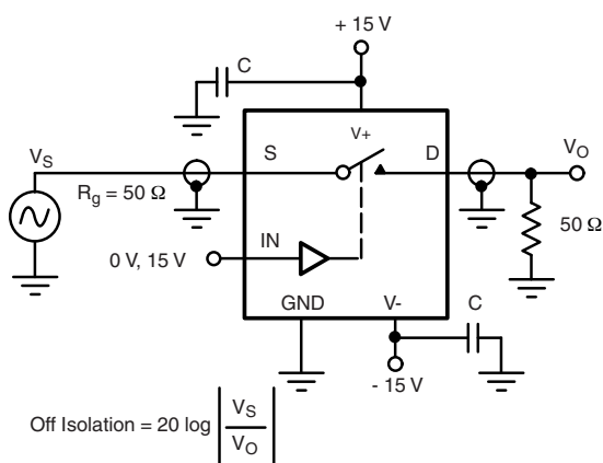
Figure 3. Off Isolation
