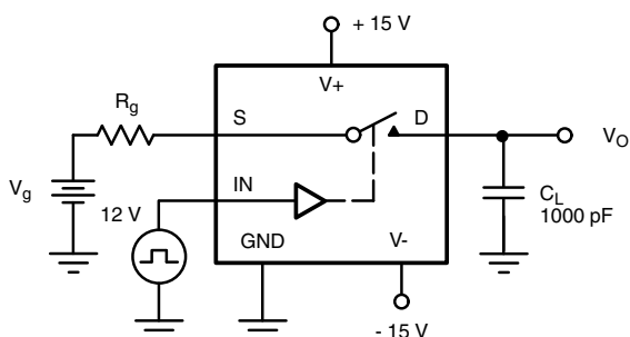
Figure 5. Charge Injection
