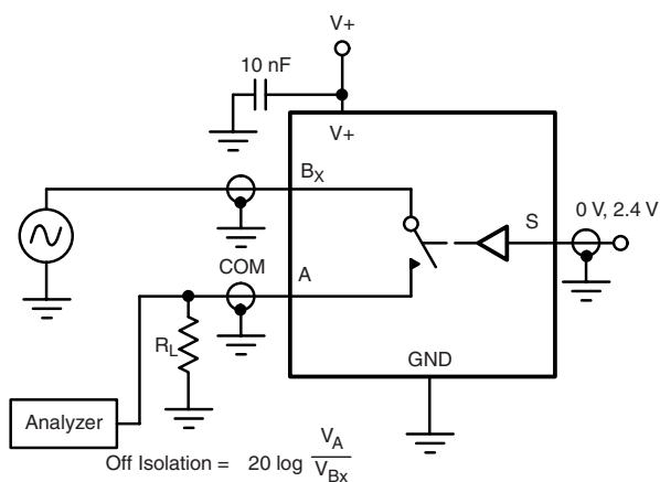
Figure 6. Off-Isolation
