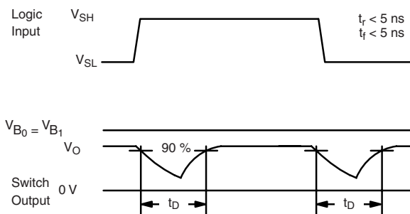
Figure 4. Break-Before-Make Interval
