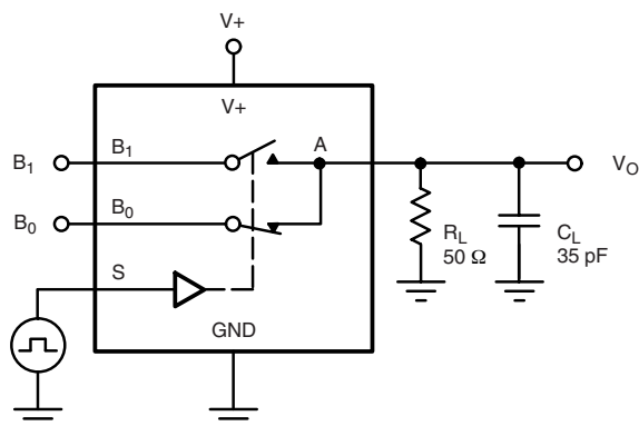
Figure 4. Break-Before-Make Interval
