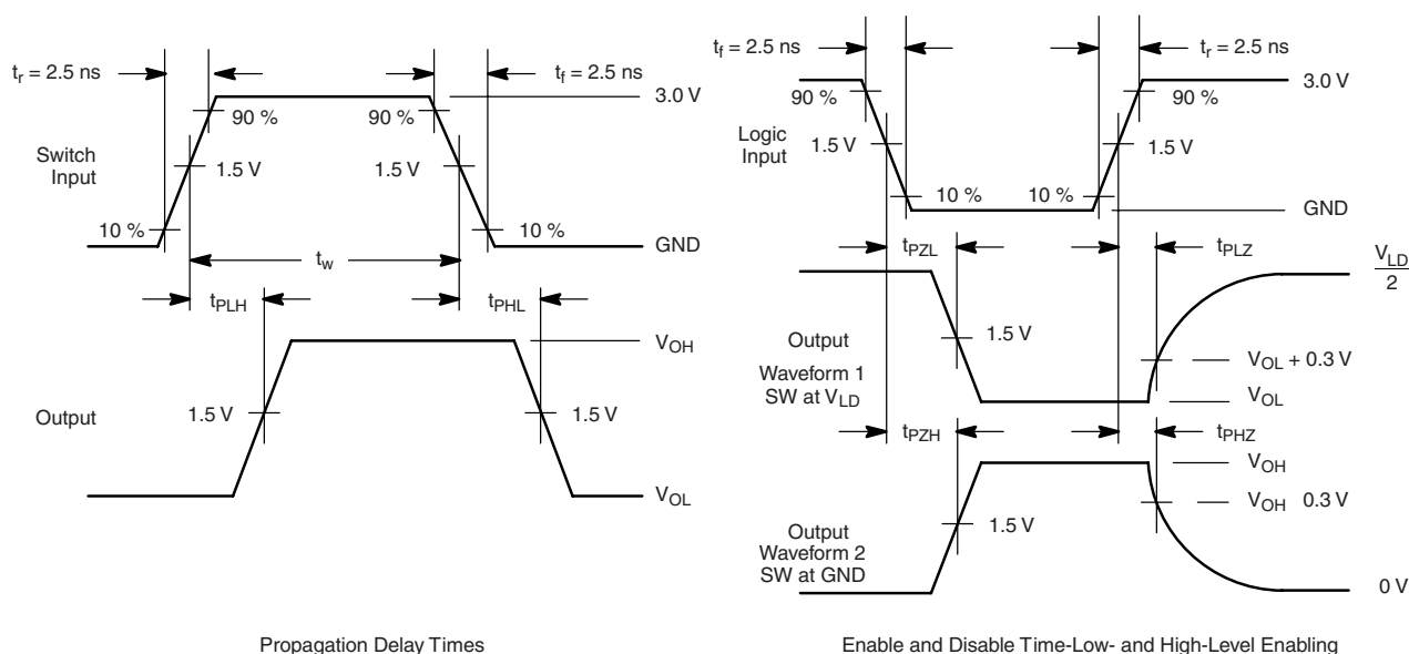
Figure 3. AC Waveforms
