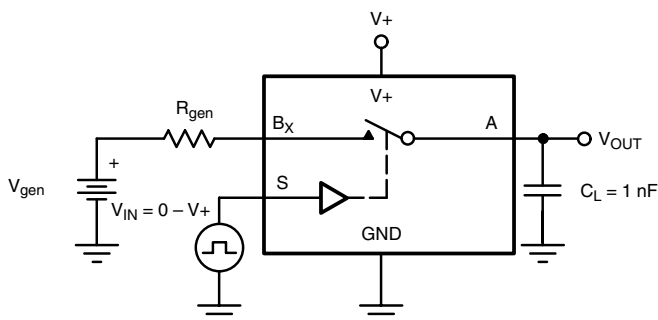
Figure 5. Charge Injection
