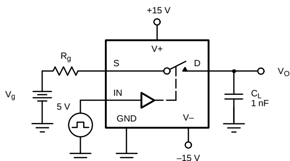
FIGURE 4. Charge Injection
