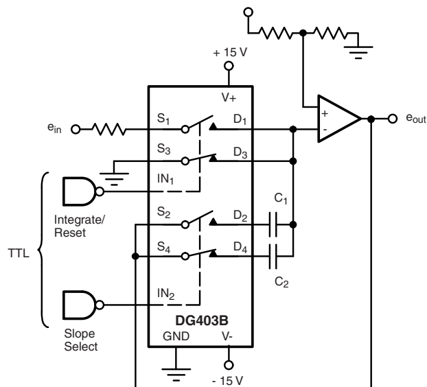
Figure 10. Dual Slope Integrator
