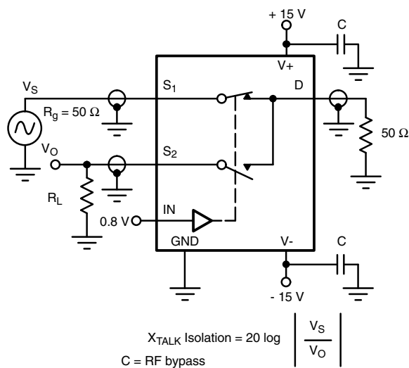
Figure 7. Crosstalk
