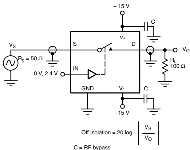
Figure 5. Off Isolation
