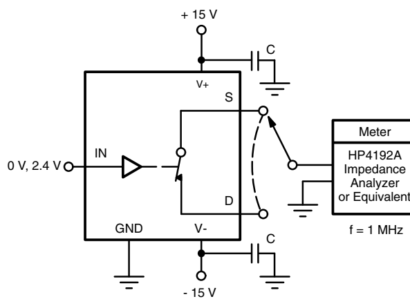
Figure 8. Capacitances
