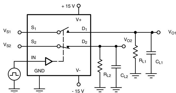
Figure 3. Break-Before-Make
