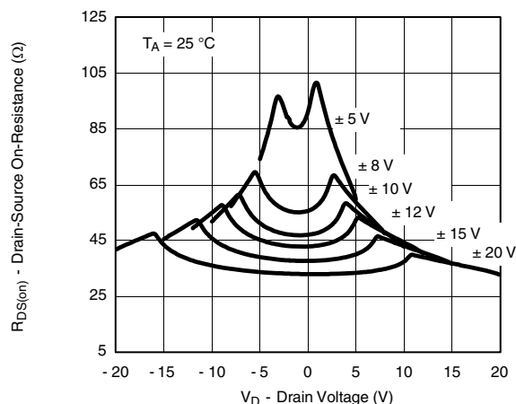
On-Resistance vs. V_D and Dual Supply Voltage
