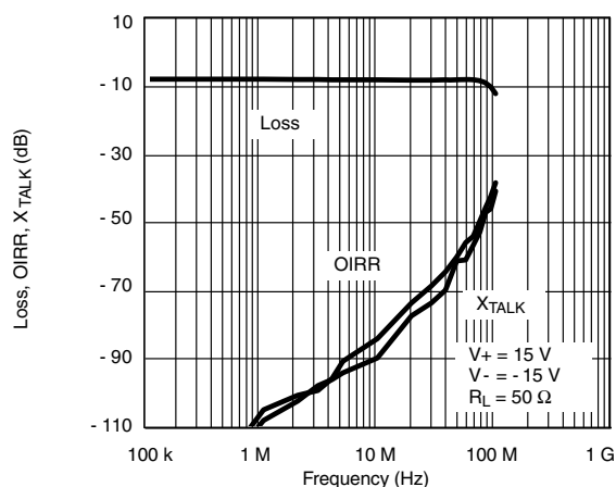
Insertion Loss, Off-Isolation Crosstalk vs. Frequency
