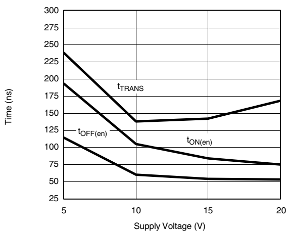
Switching Time vs. Single Supplies
