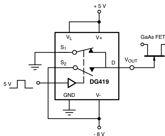
Figure 13. GaAs FET Driver
