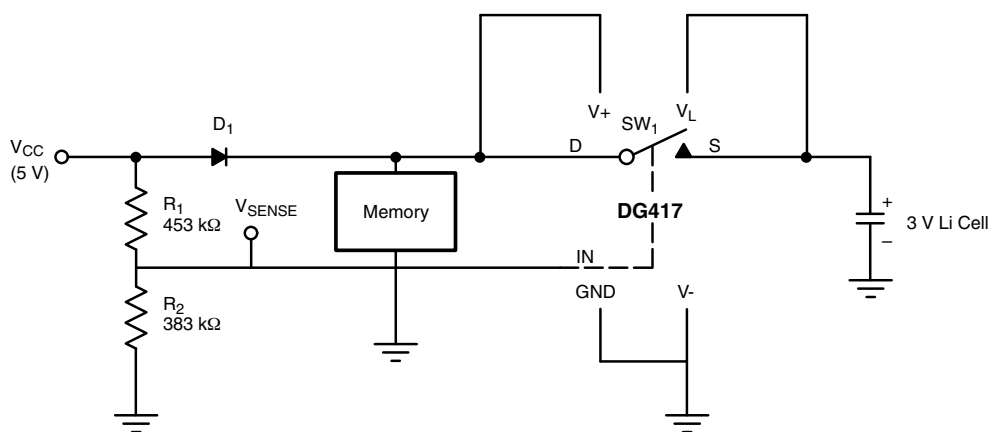
Figure 11. Micropower UPS Circuit
