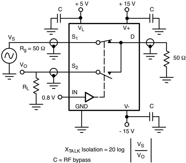
Figure 6. Crosstalk (DG419)
