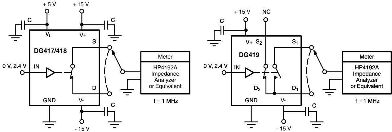
Figure 9. Source/Drain Capacitances
