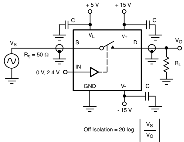
Figure 7. Off Isolation
