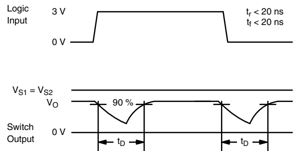
Figure 3. Break-Before-Make (DG419)
