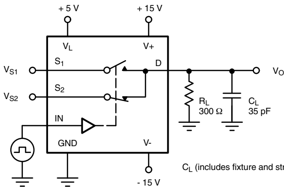
Figure 3. Break-Before-Make (DG419)
