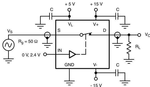
Figure 8. Insertion Loss
