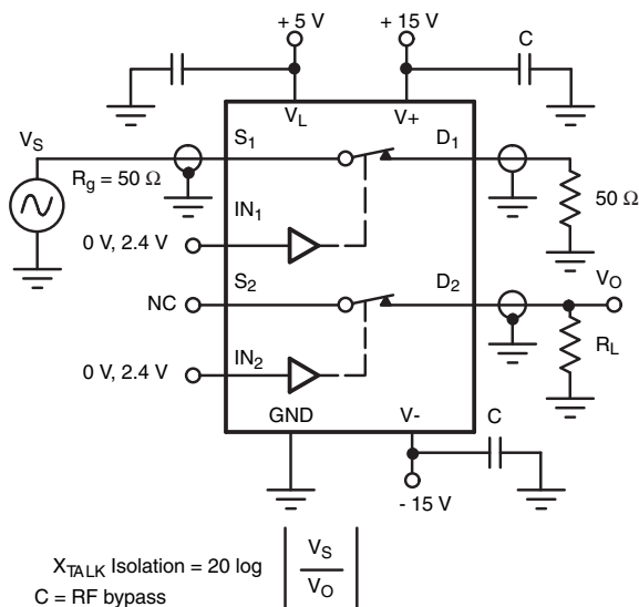
Figure 4. Crosstalk
