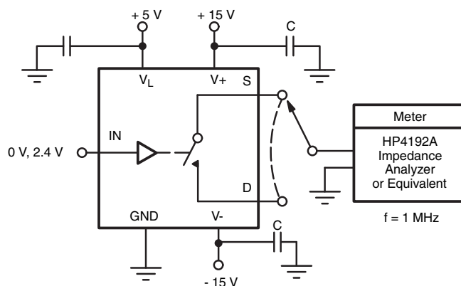
Figure 6. Source/Drain Capacitances
