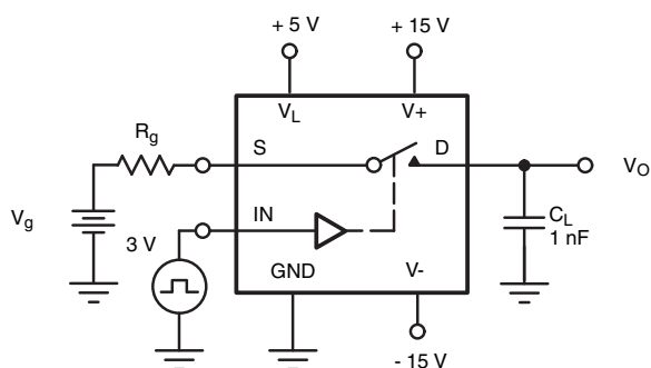
Figure 3. Charge Injection
