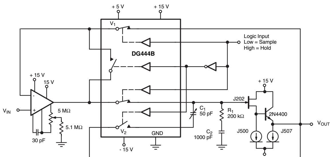
Figure 9. Precision Sample-and-Hold
