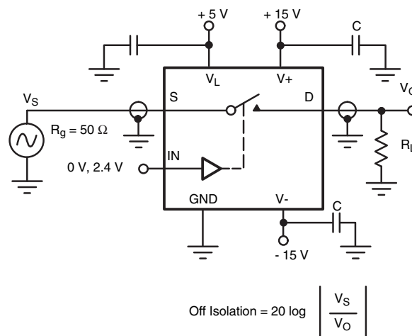
Figure 5. Off Isolation
