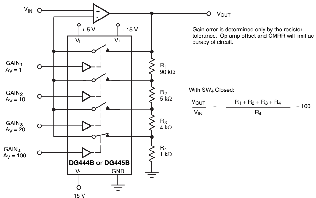
Figure 8. Precision-Weighted Resistor Programmable-Gain Amplifier
