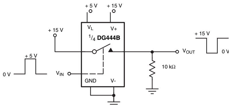
Figure 7. Level Shifter
