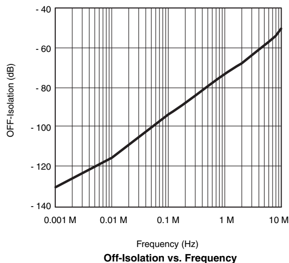
Off-Isolation vs. Frequency
