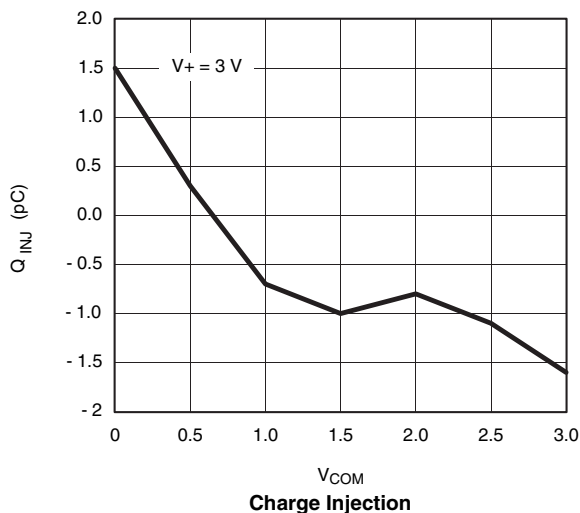
Charge Injection
