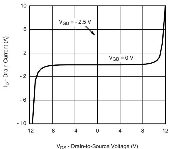
Bi-Directional Blocking Drain-Source Voltage
