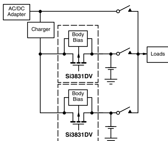
Figure 1. Charger Demultiplexing
