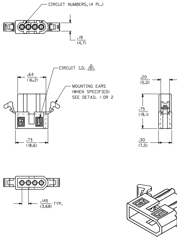
PLUG HOUSING
