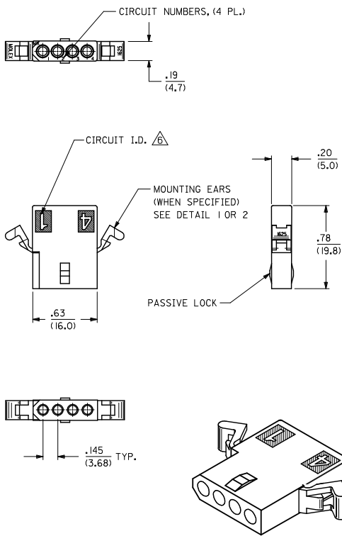
RECEPTACLE HOUSING
