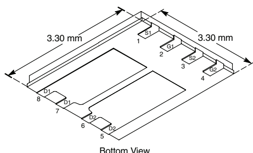
PowerPAK® 1212-8
