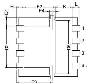
Backside view of single pad
