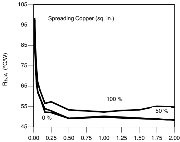
Figure 5. Spreading Copper - Si7401DN
