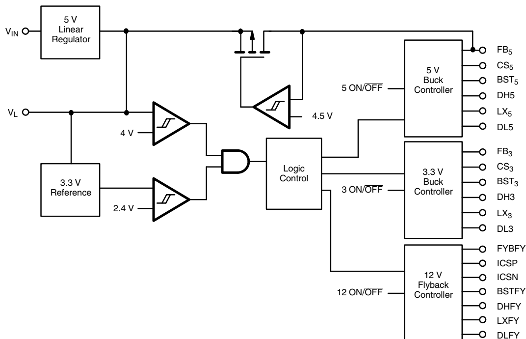
Figure 7. Complete Si9136 Block Diagram
