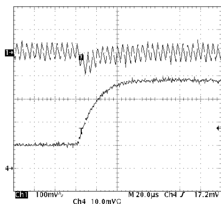
PWM, Loading 3 V Converter ( V_{IN} = 10\text{ V} )
