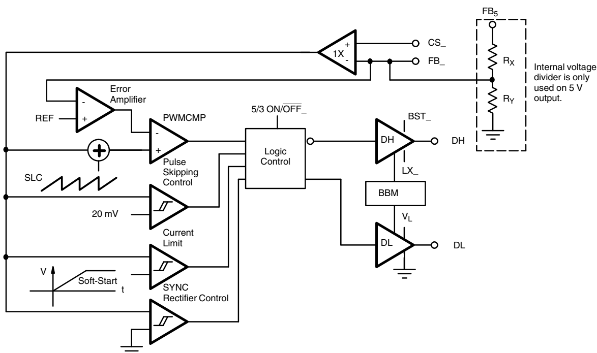
Figure 5. Buck Block Diagram
