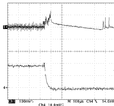
PWM \rightarrow PSM 5 V Converter ( V_{IN} = 10\text{ V} )
