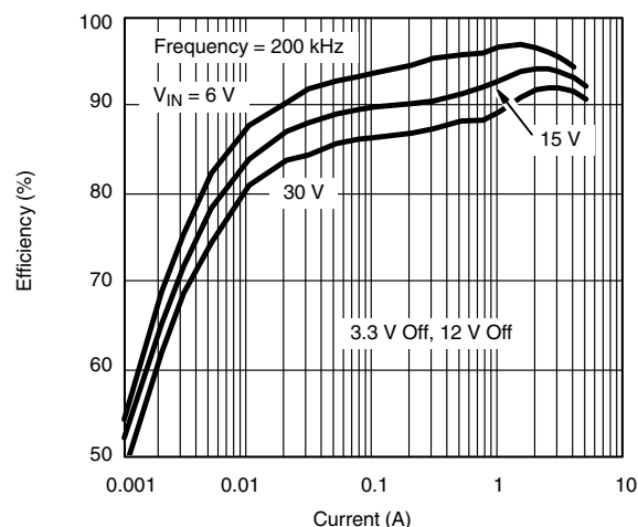
Efficiency vs. 5.0 V Output Current
