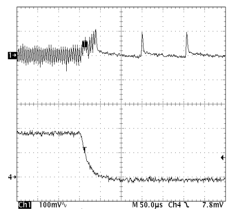
PWM \rightarrow PSM 3 V Converter ( V_{IN} = 10\text{ V} )
