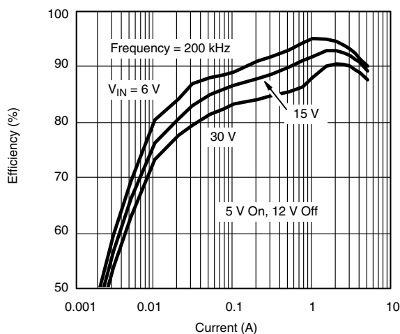
Efficiency vs. 3.3 V Output Current
