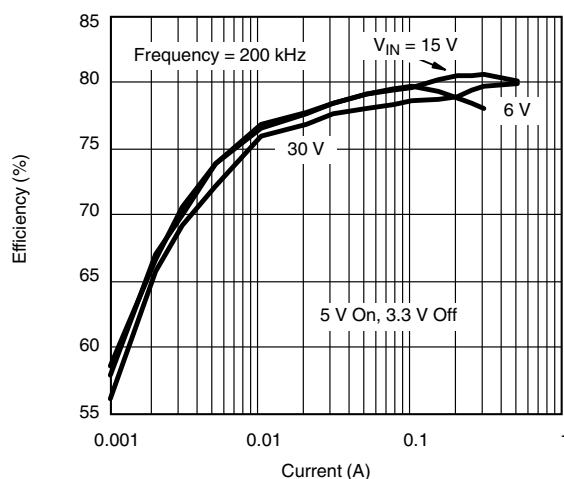
Efficiency vs. 12 V Output Current
