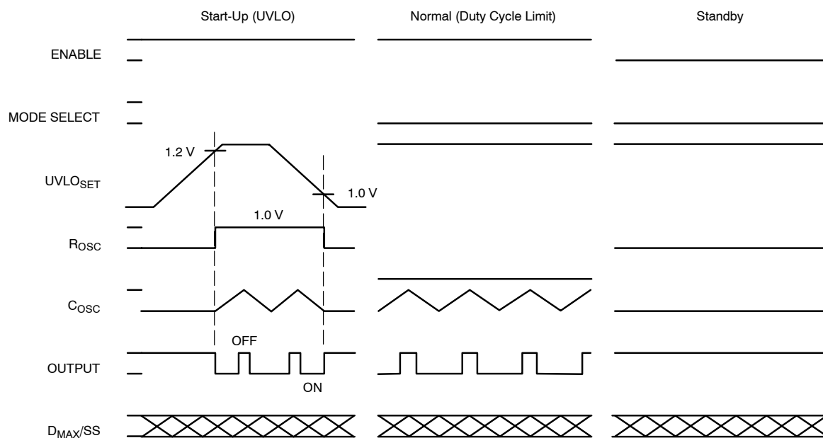
Figure 2. Si9145 Timing Diagram (MODE SELECT = Low)
