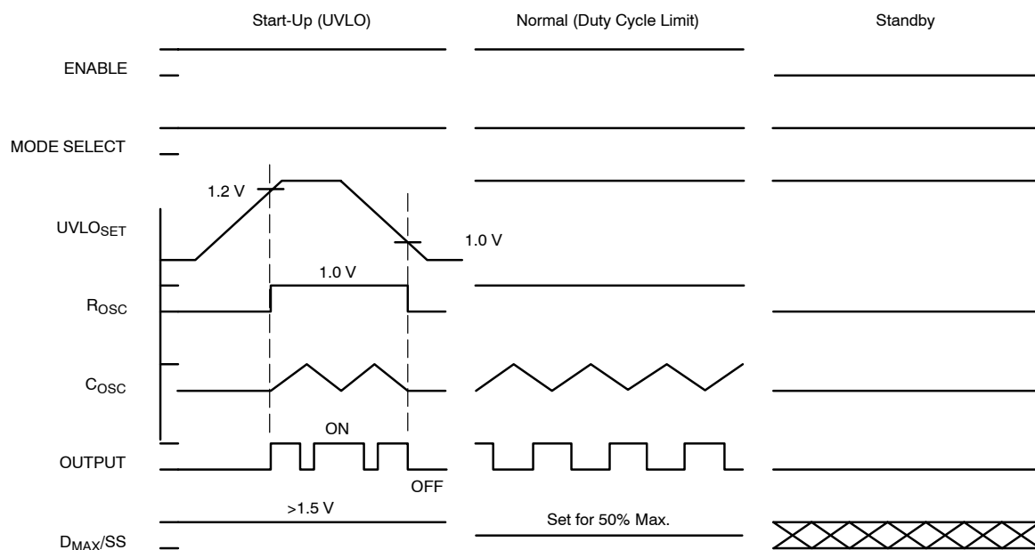
Figure 1. Si9145 Timing Diagram (MODE SELECT = High)
