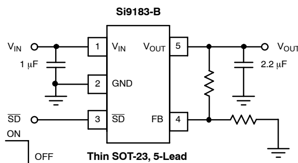
FIGURE 2. Version B with Adjustable Output
