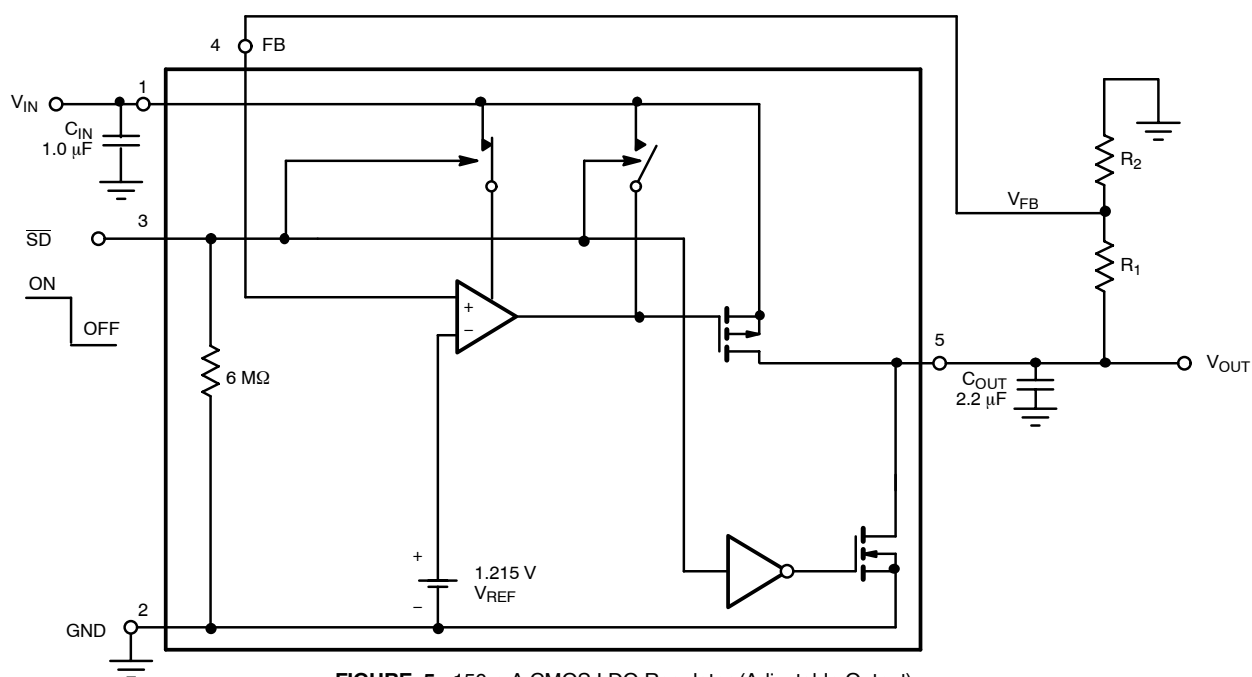
FIGURE 5. 150-mA CMOS LDO Regulator (Adjustable Output)
