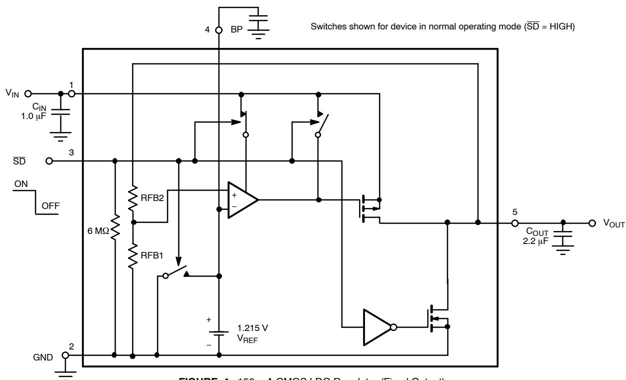
FIGURE 4. 150-mA CMOS LDO Regulator (Fixed Output)
