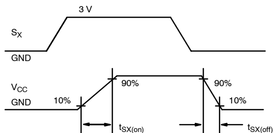
FIGURE 1. Switch Ramp
