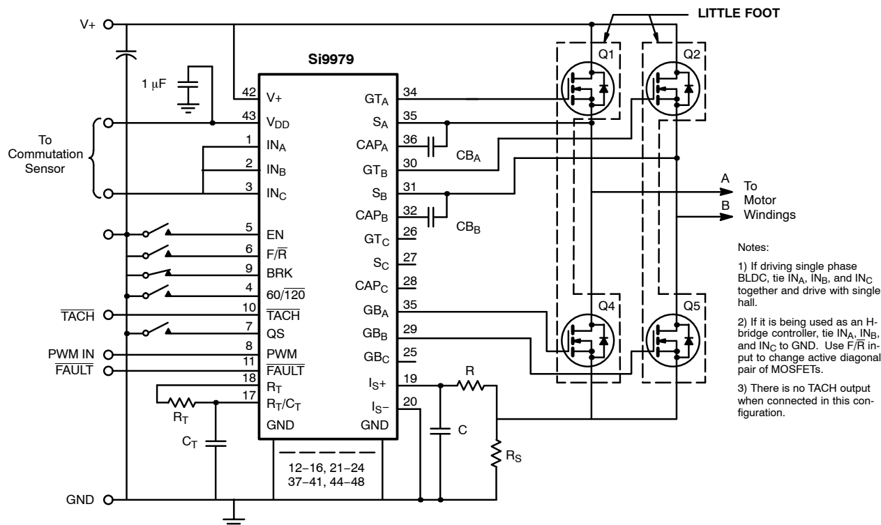
FIGURE 2. Single H-Bridge Controller
