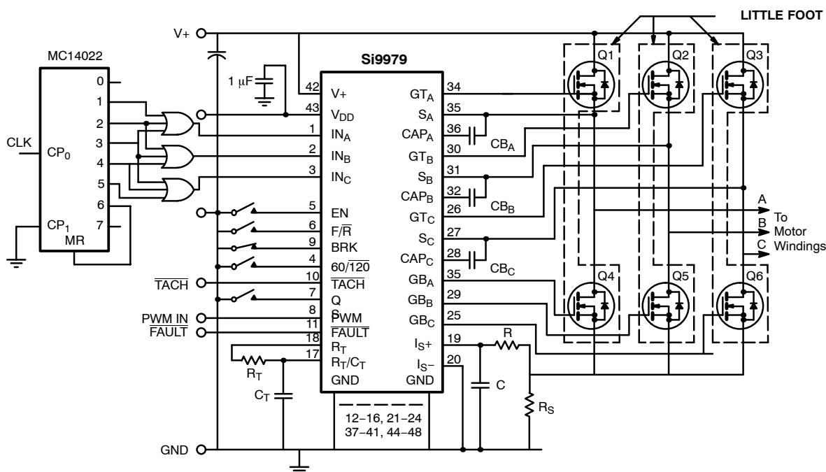
FIGURE 3. Three-Phase AC Motor Controller
