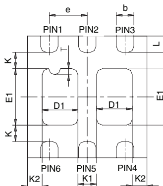
BACKSIDE VIEW OF DUAL
