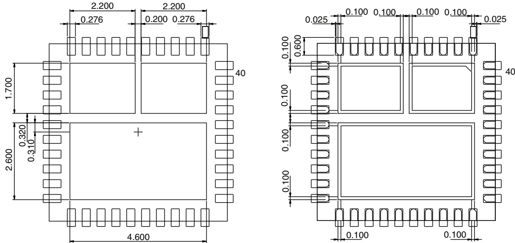
Figure 9 - PowerPAK MLP 66-40
