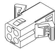
DETAIL 2 RECEPTACLE WITHOUT EARS OR DETENTS, ENG. NO. 2004-R3*
