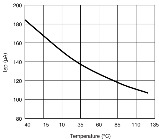
I SD vs. Temperature
