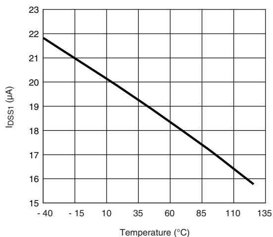
I DSS1 vs. Temperature
