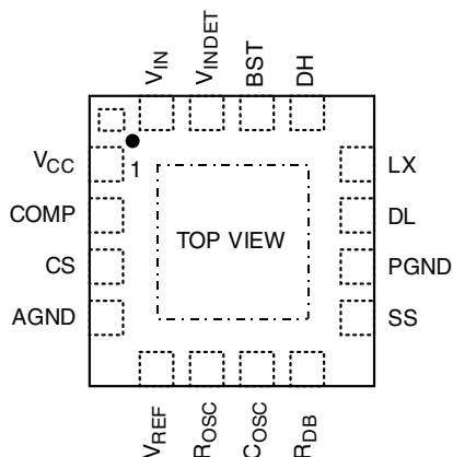
MLP44-16 PowerPAK Package
