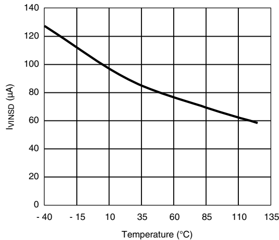
I VNSD vs. Temperature
