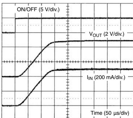
SiP4280-3 Turn-On ( V_{IN} = 5 V, R_{LOAD} = 10 \Omega )
