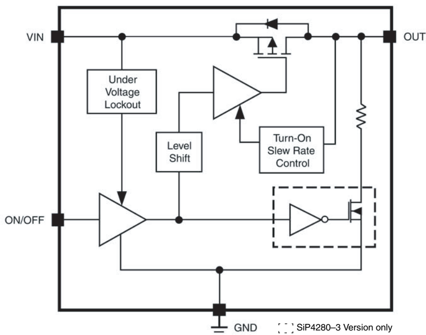
SiP4280 Functional Block Diagramm
