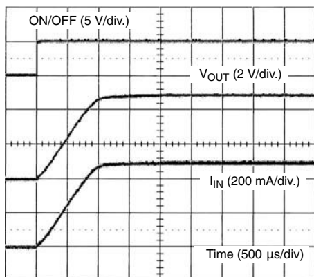
SiP4280-1 Turn-On ( V_{IN} = 5 V, R_{LOAD} = 10 \Omega )
