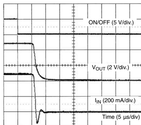
SiP4280-1 Turn-Off ( V_{IN} = 5 V, R_{LOAD} = 10 \Omega )
