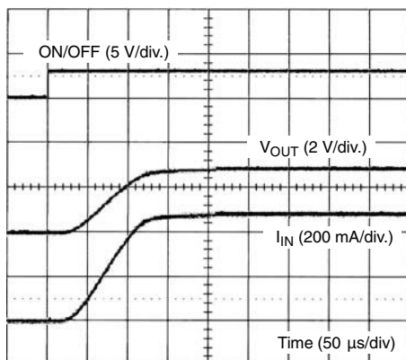
SiP4280-3 Turn-On ( V_{IN} = 3 V, R_{LOAD} = 6 \Omega )
