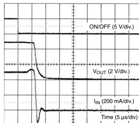
SiP4280-3 Turn-Off ( V_{IN} = 5 V, R_{LOAD} = 10 \Omega )
