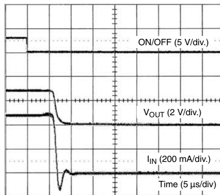
SiP4280-1 Turn-Off ( V_{IN} = 3 V, R_{LOAD} = 6 \Omega )
