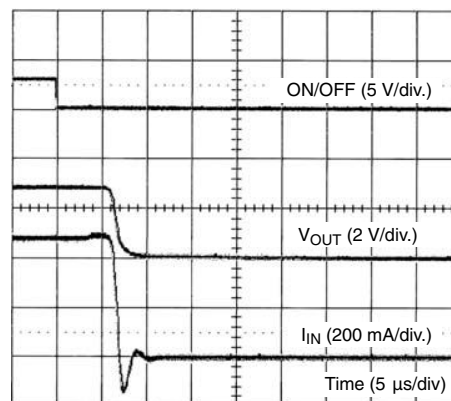
SiP4280-3 Turn-Off ( V_{IN} = 3 V, R_{LOAD} = 6 \Omega )
