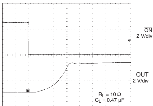
10 \mu\text{s/div} Turn On
