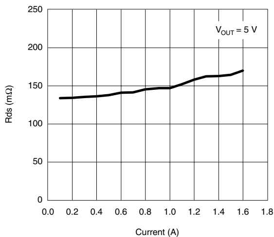
Rds ( V_{OUT} to V_{IN} ) vs. Current
