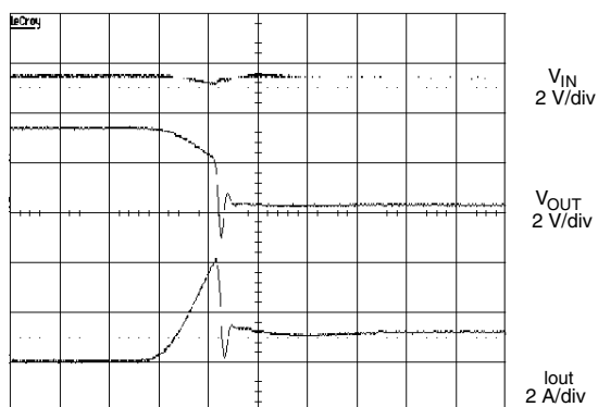
2 \mu\text{s/div} Short Circuit through 0.3 \Omega , V_{in} = 3.3\text{ V}
