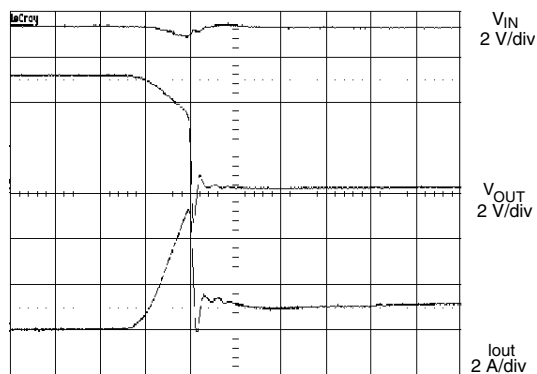
2 \mu\text{s/div} Short Circuit through 0.3 \Omega , V_{in} = 5\text{ V}
