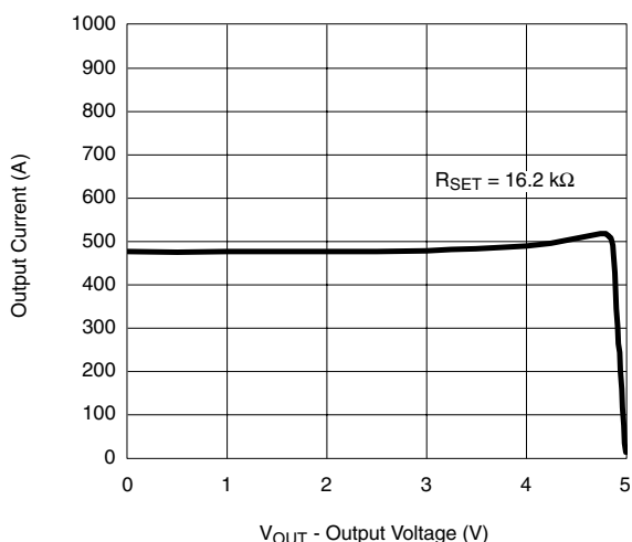
Output Current vs. V OUT
