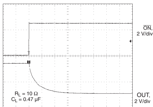
10 \mu\text{s/div} Turn Off
