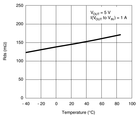
Rds ( V_{OUT} to V_{IN} ) vs. Temperature
