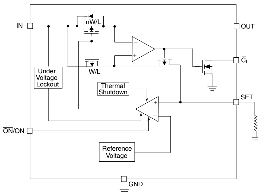
Figure 1. SiP4613A/B Block Diagram
