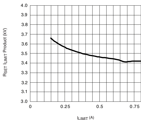
R_{\text{SET}} Coefficient vs. I_{\text{LIMIT}}
