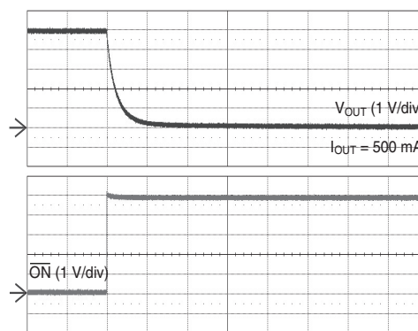
Turn Off
