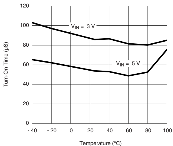
Turn-On vs. Temperature R_{\text{L}} = 10\ \Omega , C_{\text{L}} = 0.47\ \mu\text{F}
