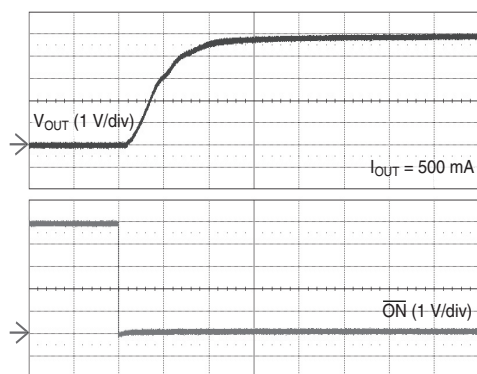
Turn On
