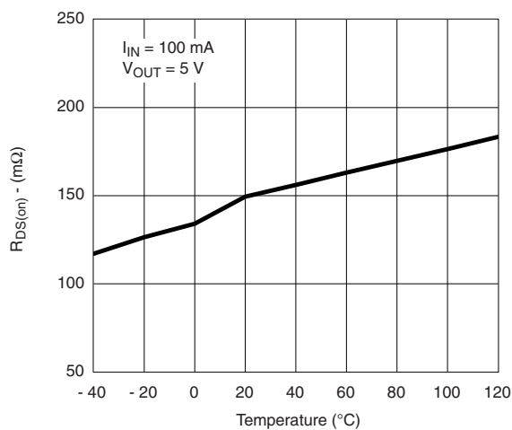
R_{DS(on)} _reverse vs. Temperature
