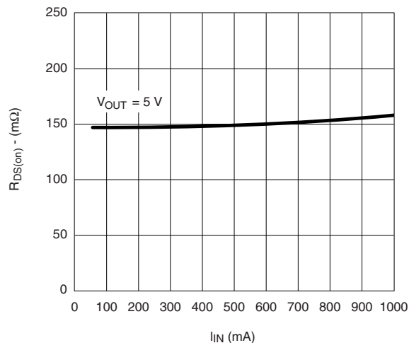
R_{DS(VOUT-IN)} vs. Current
