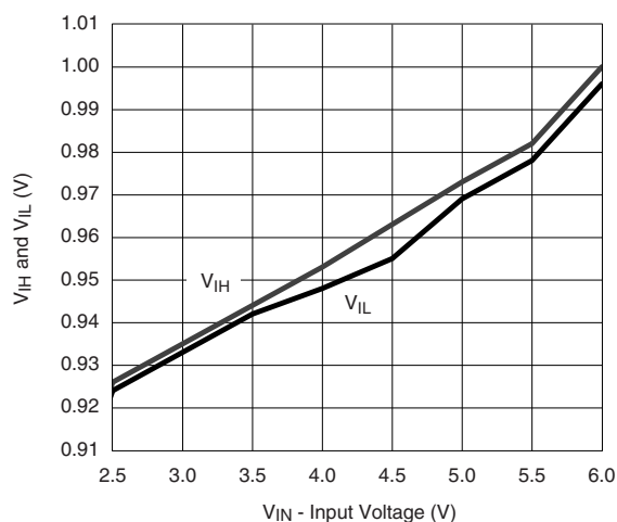
V_{\text{IH}} and V_{\text{IL}} vs. V_{\text{IN}}
