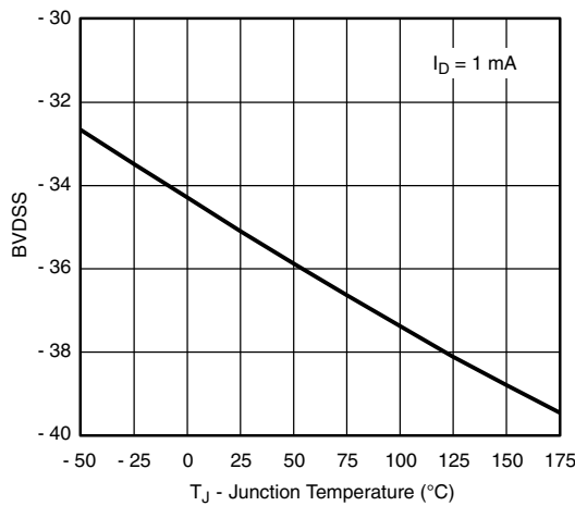
BVDS vs. Junction Temperature
