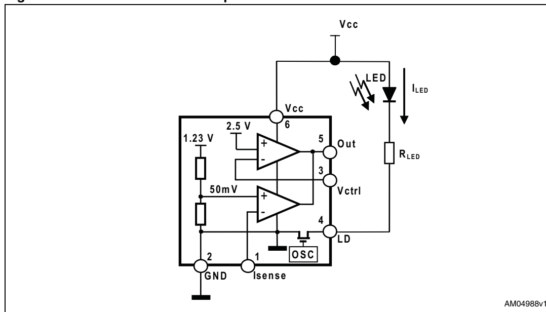
Figure 5. Connection of LED to pin LD
