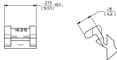
DETAIL B
