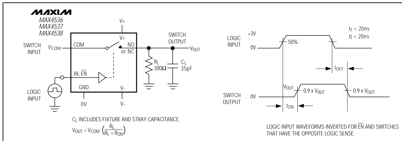
Figure 1. Switching Time
