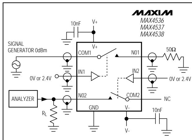
Figure 5. Crosstalk
