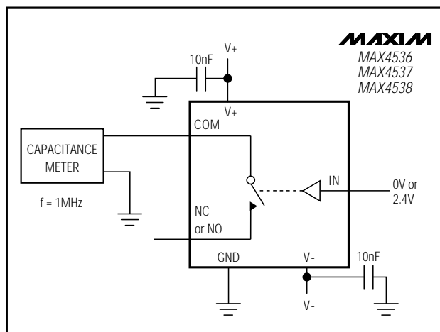
Figure 7. Channel-On Capacitance
