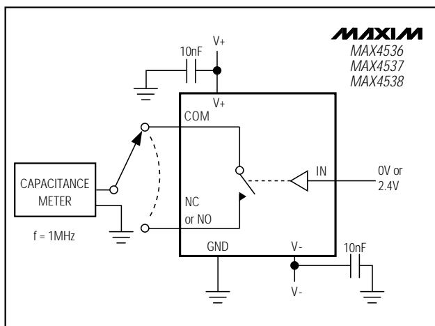
Figure 6. Channel-Off Capacitance
