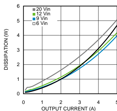
Figure 26. Dissipation 2.5-V Output at 85°C Ambient
