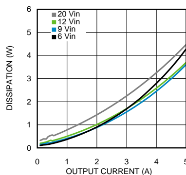
Figure 4. Dissipation 5-V Output at 25°C Ambient
