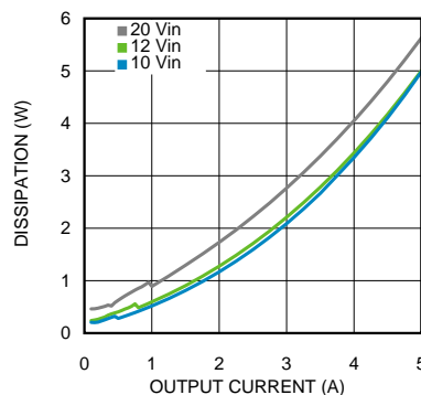
Figure 20. Dissipation 6-V Output at 85°C Ambient
