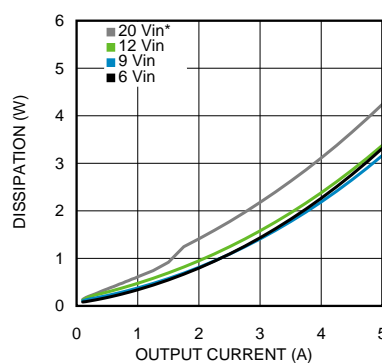
Figure 16. Dissipation 1-V Output at 25°C Ambient
