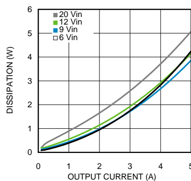
Figure 28. Dissipation 1.8-V Output at 85°C Ambient
