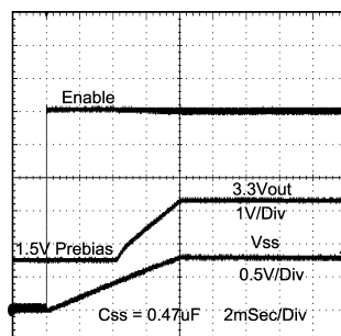
Figure 44. Prebiased Start-Up
