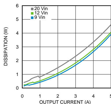
Figure 2. Dissipation 6-V Output at 25°C Ambient
