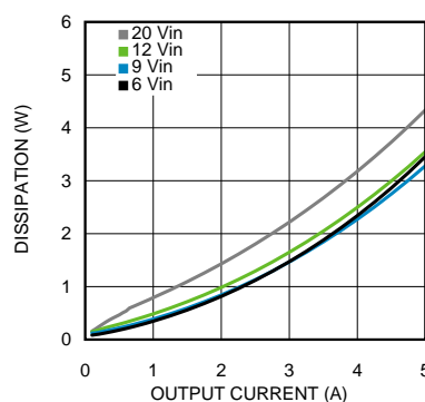
Figure 14. Dissipation 1.2-V Output at 25°C Ambient
