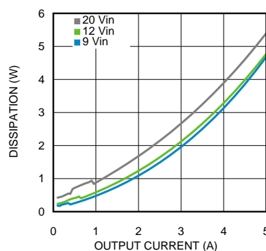
Figure 20. Dissipation 6-V Output at 85°C Ambient
