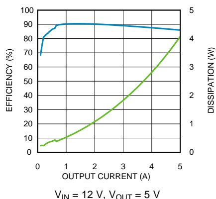
Figure 49. Efficiency
