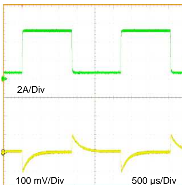
Figure 40. Output Ripple
