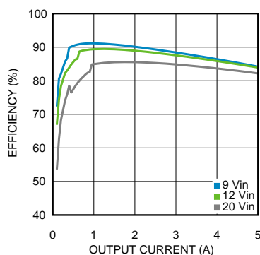
Figure 19. Efficiency 6-V Output at 85°C Ambient
