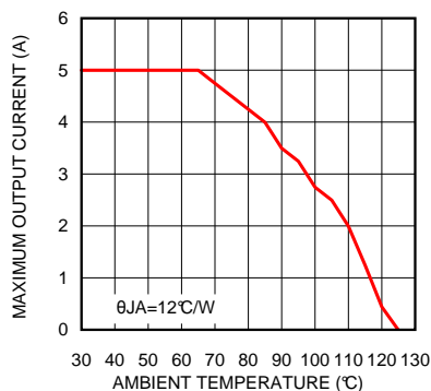
Figure 37. Thermal Derating
