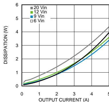
Figure 8. Dissipation 2.5-V Output at 25°C Ambient
