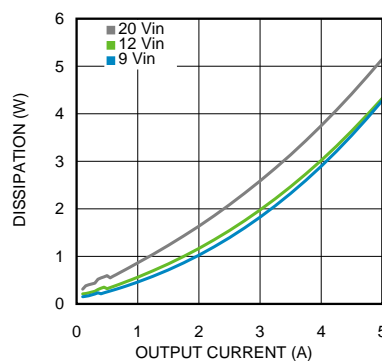
Figure 22. Dissipation 5-V Output at 85°C Ambient
