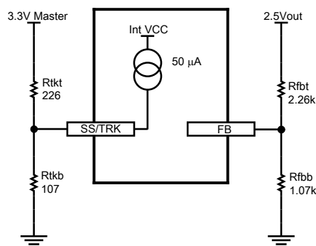
Figure 48. Tracking Option Input Detail
