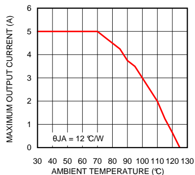
Figure 38. Thermal Derating
