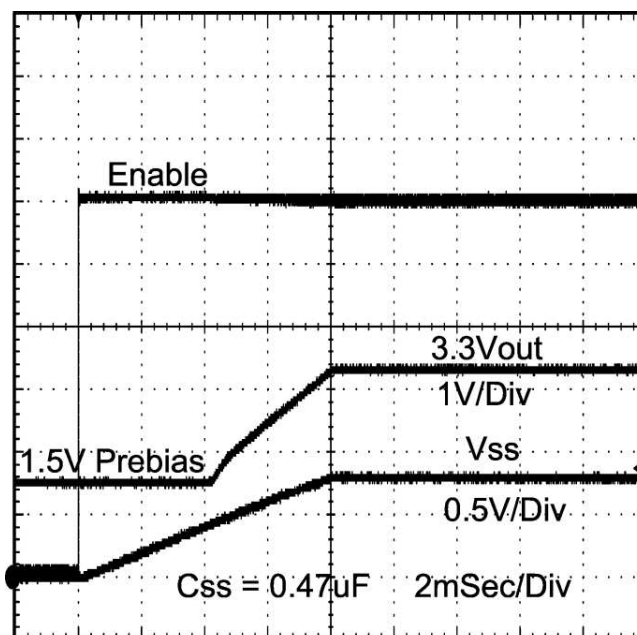
Figure 46. Prebiased Start-Up
