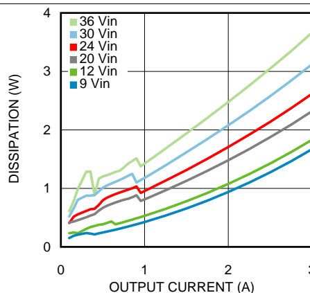
Figure 2. Dissipation 6-V Output at 25°C Ambient
