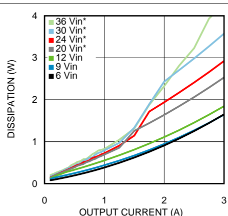
Figure 34. Dissipation 1-V Output at 85°C Ambient
