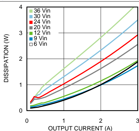
Figure 26. Dissipation 2.5-V Output at 85°C Ambient
