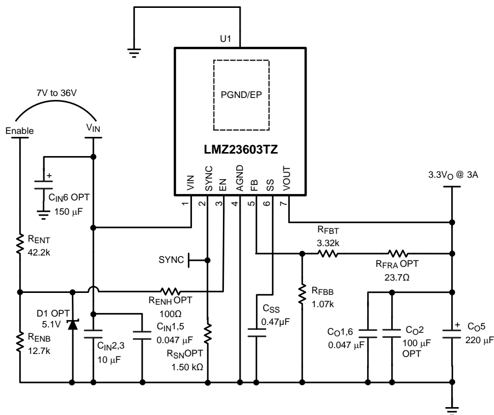
Figure 48. Simplified Evaluation Board Schematic Diagram
