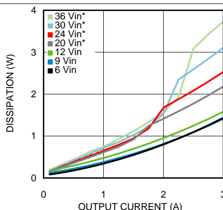
Figure 16. Dissipation 1-V Output at 25°C Ambient
