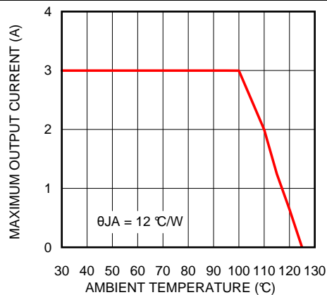
Figure 38. Thermal Derating
