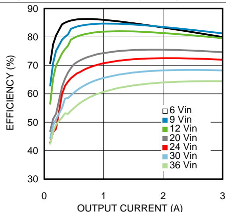
Figure 25. Efficiency 2.5-V Output at 85°C Ambient
