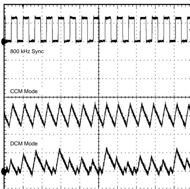
Figure 47. CCM and DCM Operating Modes
