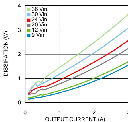
Figure 4. Dissipation 5-V Output at 25°C Ambient
