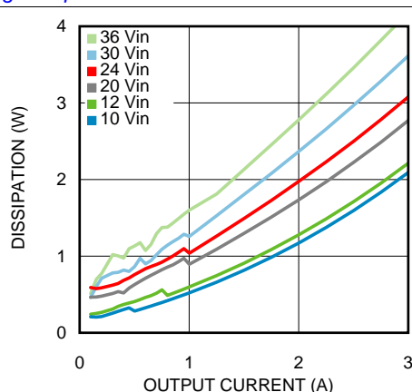
Figure 20. Dissipation 6-V Output at 85°C Ambient
