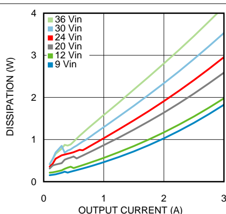
Figure 22. Dissipation 5-V Output at 85°C Ambient
