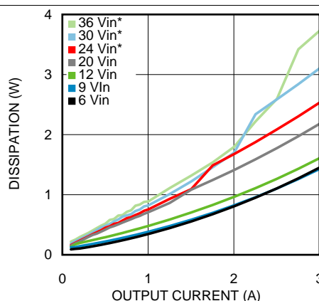
Figure 14. Dissipation 1.2-V Output at 25°C Ambient
