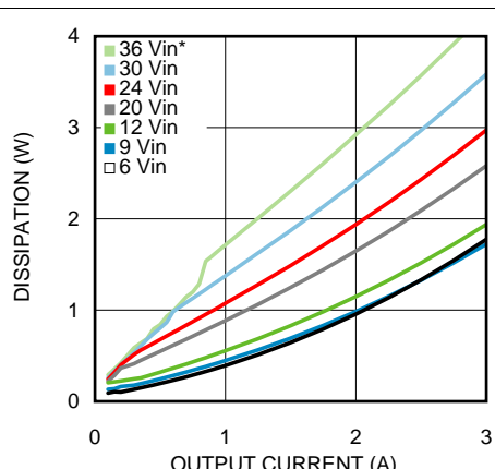
Figure 26. Dissipation 2.5-V Output at 85°C Ambient
