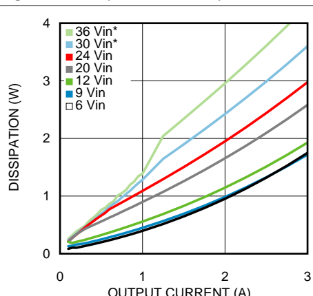
Figure 28. Dissipation 1.8-V Output at 85°C Ambient
