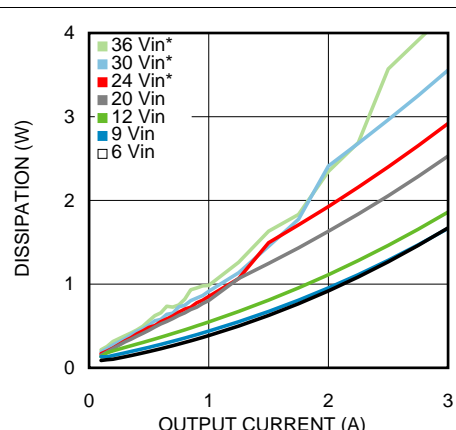
Figure 32. Dissipation 1.2-V Output at 85°C Ambient
