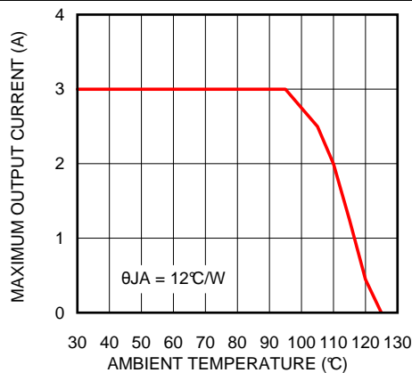
Figure 37. Thermal Derating
