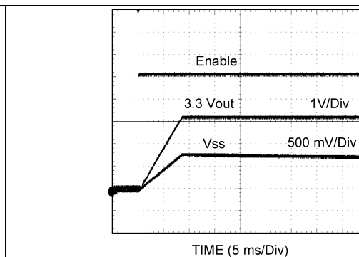
Figure 44. 3.3 V_{OUT} Soft-Start
