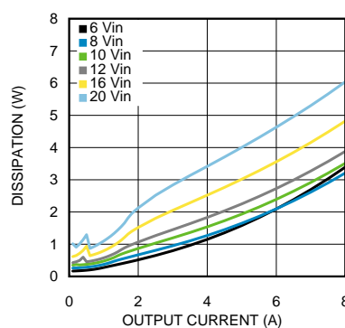
Figure 16. Dissipation 5-V Output at 85°C
