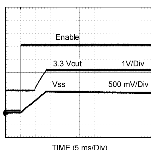
Figure 48. Prebiased Start-Up
