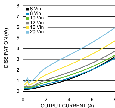
Figure 20. Dissipation 2.5-V Output at 85°C
