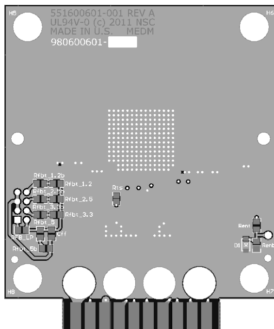
Figure 59. Bottom View of Evaluation PCB
