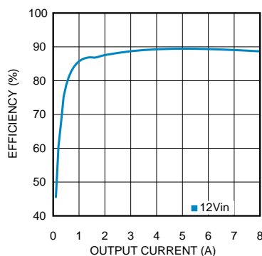
Figure 53. Efficiency
