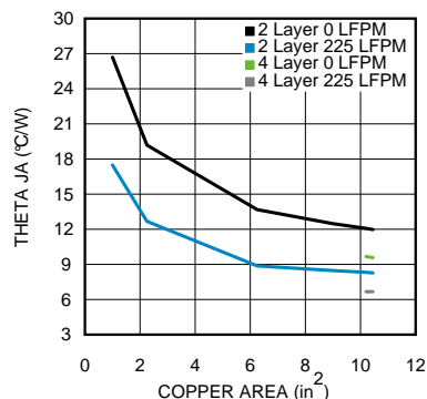
Figure 32. R_{\theta JA} vs Copper Heat Sinking Area
