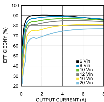
Figure 19. Efficiency 2.5-V Output at 85°C
