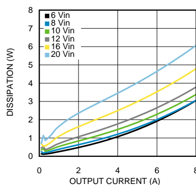
Figure 26. Dissipation 1.2-V Output at 85°C
