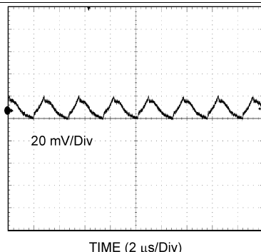
Figure 33. Output Ripple
