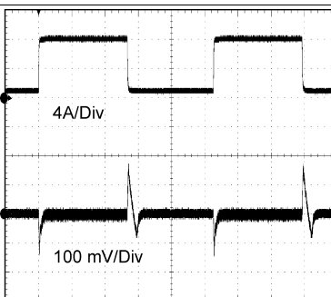
TIME (500 \mu\text{s/Div} ) 12 V_{IN} , 1.2 V_{OUT} , 1- to 8-A Step
