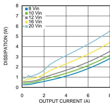
Figure 2. Dissipation 5-V Output at 25°C
