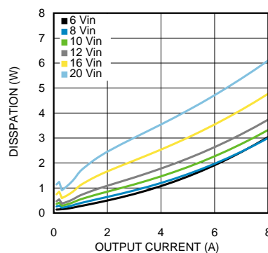
Figure 22. Dissipation 1.8-V Output at 85°C
