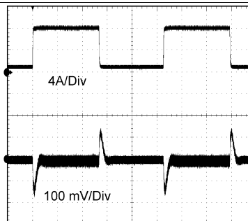
TIME (500 \mu\text{s/Div} ) 12 V_{IN} , 3.3 V_{OUT} , 1- to 8-A Step
