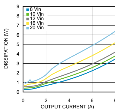
Figure 14. Dissipation 1-V Output at 25°C
