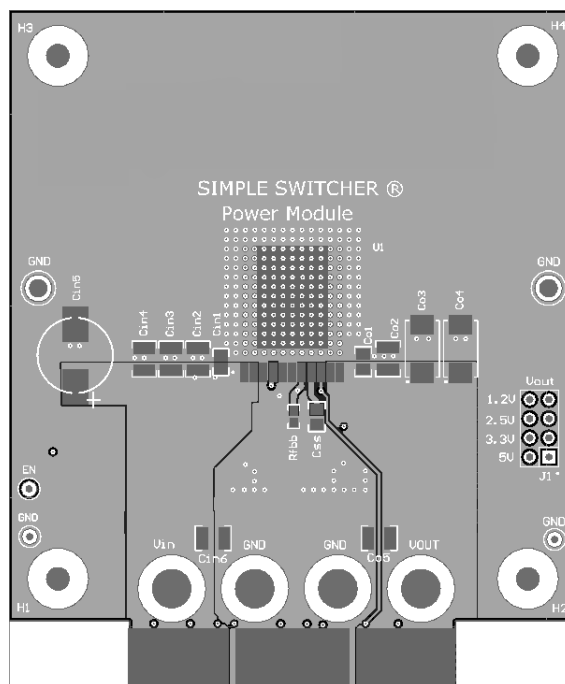
Figure 58. Top View of Evaluation PCB
