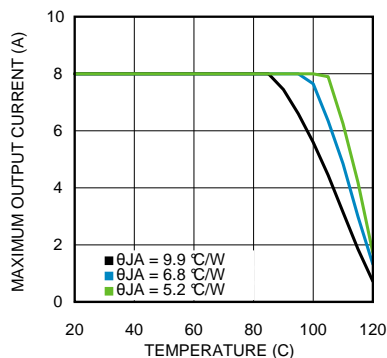
Figure 31. Thermal Derating
