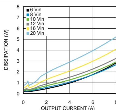
Figure 4. Dissipation 3.3-V Output at 25°C
