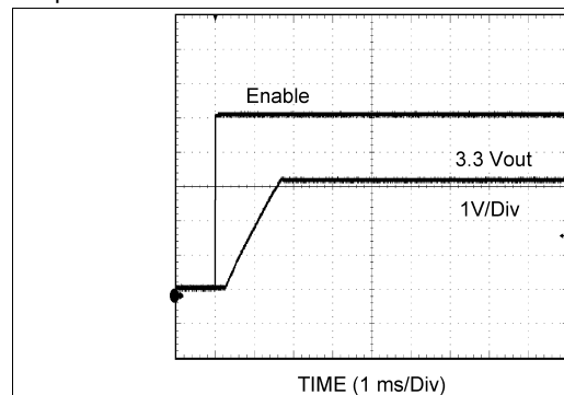
Figure 43. 3.3 V_{OUT} Soft-Start
