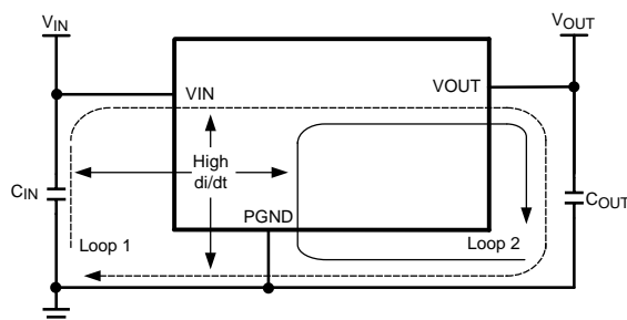
Figure 56. Critical Current Loops to Minimize
