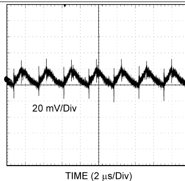
Figure 34. Output Ripple
