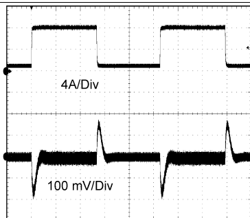
TIME (500 \mu\text{s/Div} ) 12 V_{IN} , 5 V_{OUT} , 1- to 8-A Step
