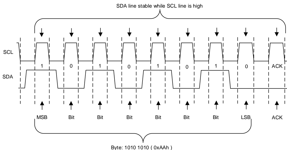
Figure 23. Definition of Byte Formation
