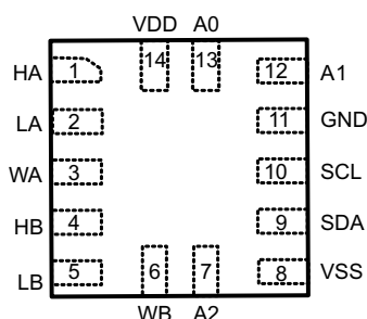
RUC Package 14-Pin MicroQFN Top View
