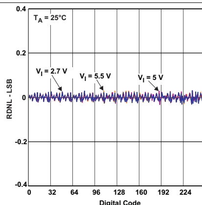
Figure 8. Rheostat Mode RDNL vs Digital Code (25°C)
