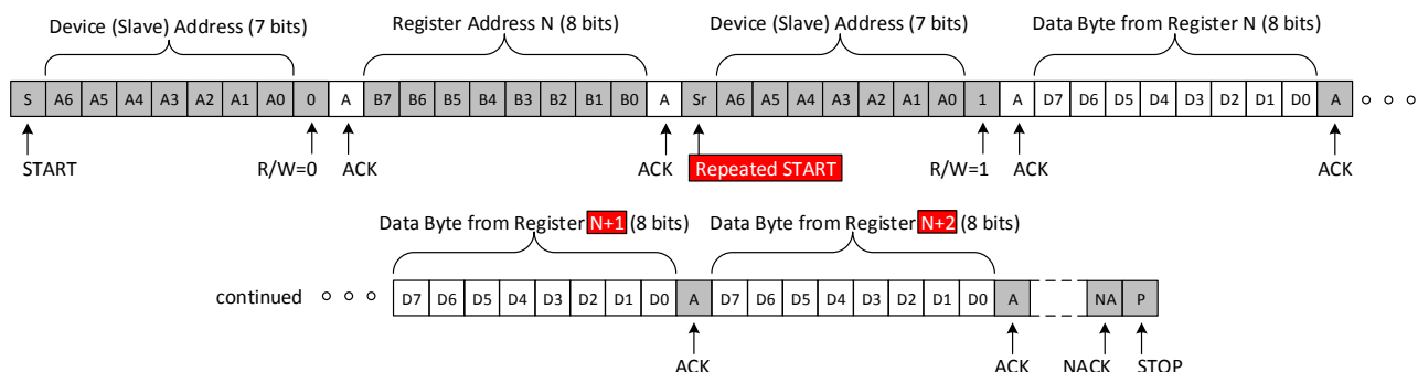
Figure 28. Read Operation from Multiple Registers
