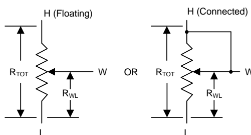
Figure 21. Equivalent Circuit for Rheostat Mode with Terminal L to Terminal W Resistance
