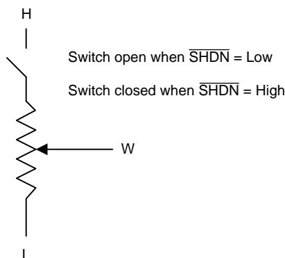
Figure 18. Equivalent Circuit for Shutdown Mode
