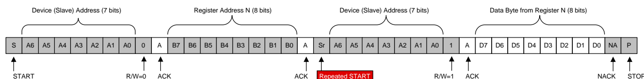
Figure 27. Read Operation from One Register
