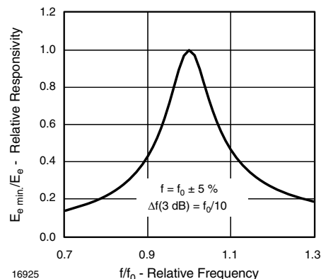
Fig. 5 - Frequency Dependence of Responsivity
