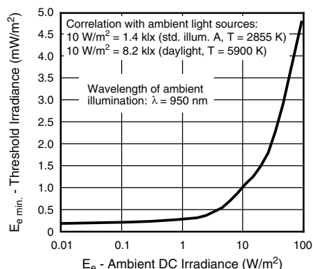
Fig. 6 - Sensitivity in Bright Ambient
