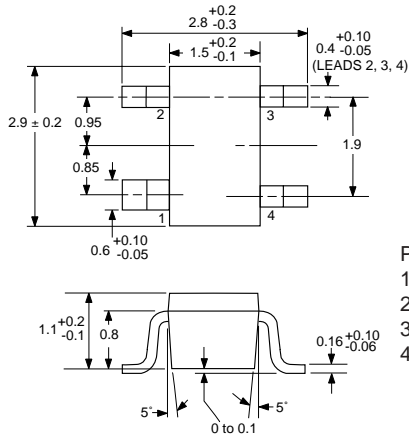
PACKAGE OUTLINE 39
