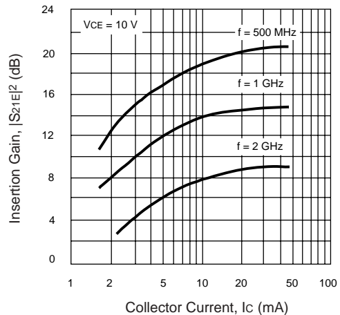
NE85635 INSERTION GAIN vs. COLLECTOR CURRENT
