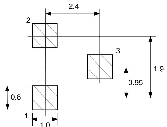
PACKAGE OUTLINE 33 RECOMMENDED P.C.B. LAYOUT
