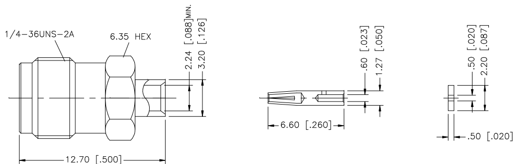
RECOMMENDED CABLE STRIPPING DIMS.
