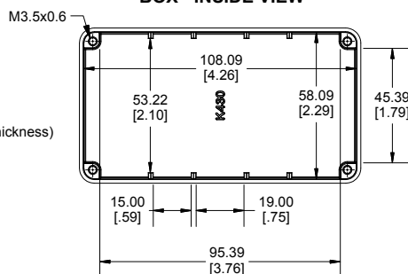
BOX - INSIDE VIEW
