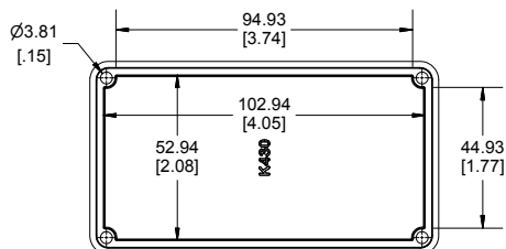
LID - INSIDE VIEW
