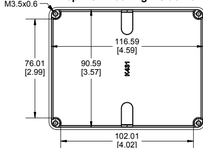
Top View Looking Inside Box
