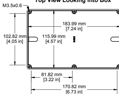
Top View Looking Into Box
