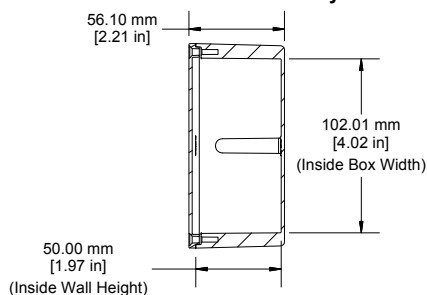
SECTION A-A End View of Assembly
