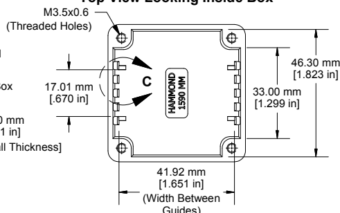
DETAIL C Top View - Interior Features
