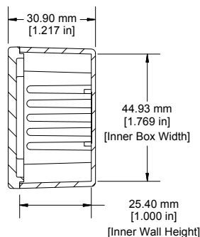
Top View Looking Inside Box
