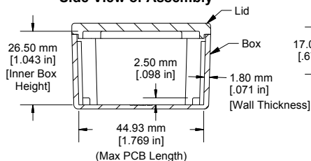
SECTION B-B Side View of Assembly
