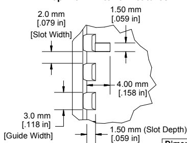
DETAIL C Top View - Interior Features
