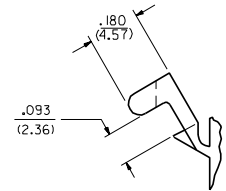
DETAIL 4 .093/(2.36) PREBENT MOUNTING EAR (SCALE 4:1)
