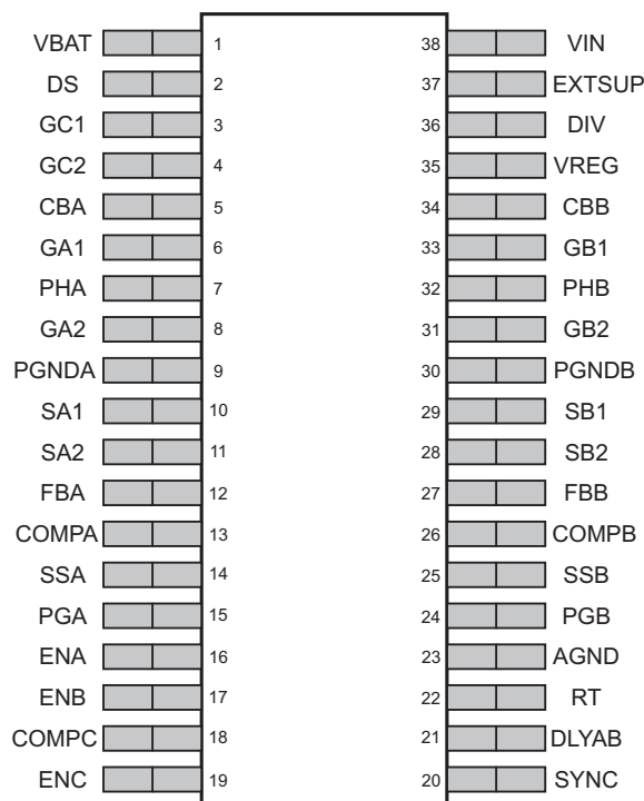
Pin Functions
