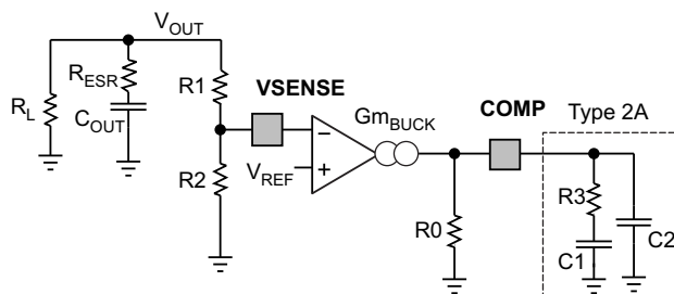
Figure 24. Buck Compensation Components
