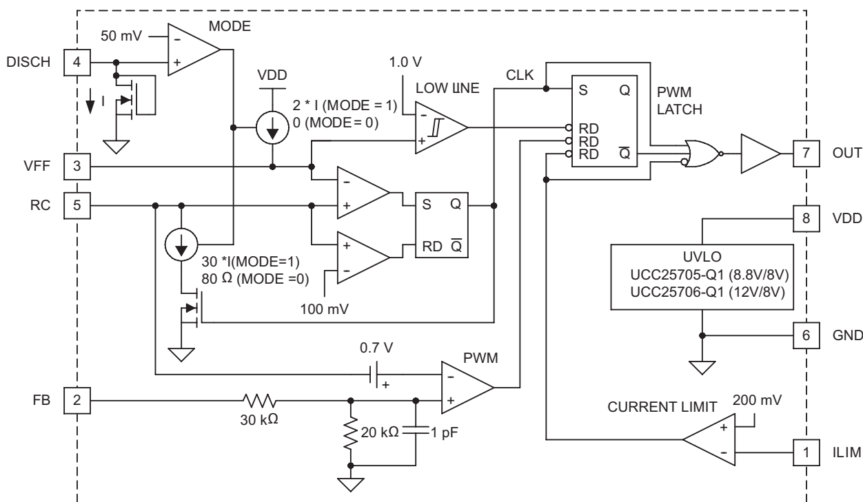
Figure 2. Block Diagram
