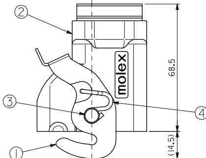
PG 29 雄ネジ PG 29 EXTERNAL THREAD
