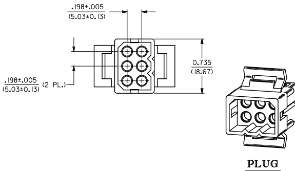
PLUG
