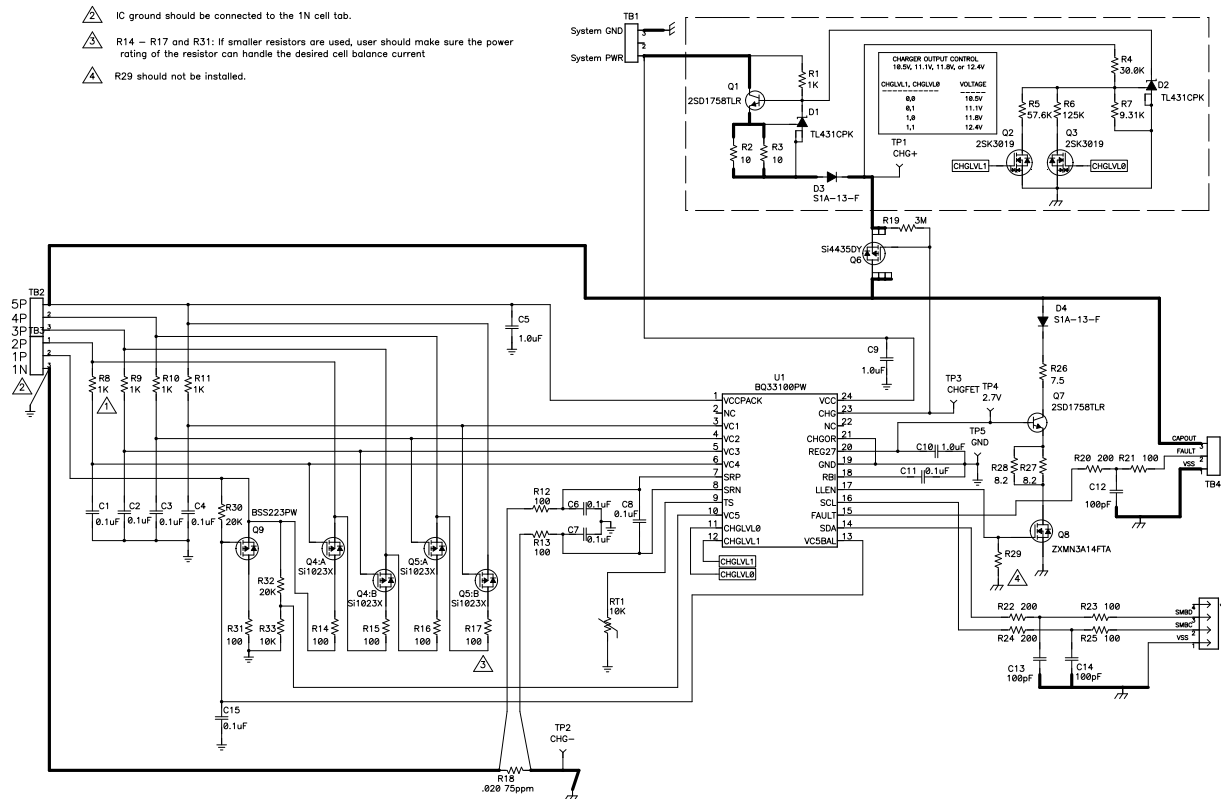
Figure 18. Application Reference Schematic
