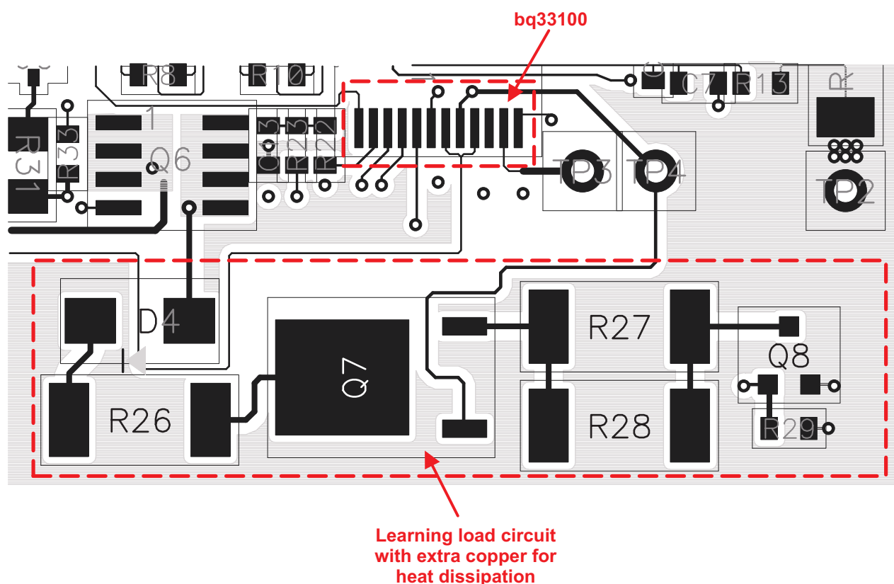
Figure 20. bq33100 Board Layout
