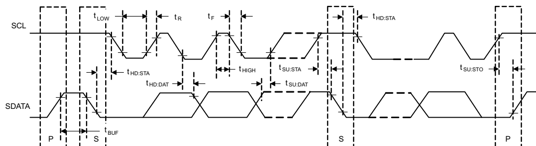
Figure 1. SMBus Timing
