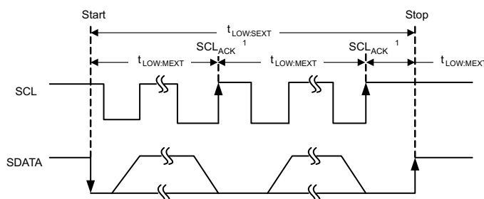
Figure 2. SMBus t_{\text{TIMEOUT}}
