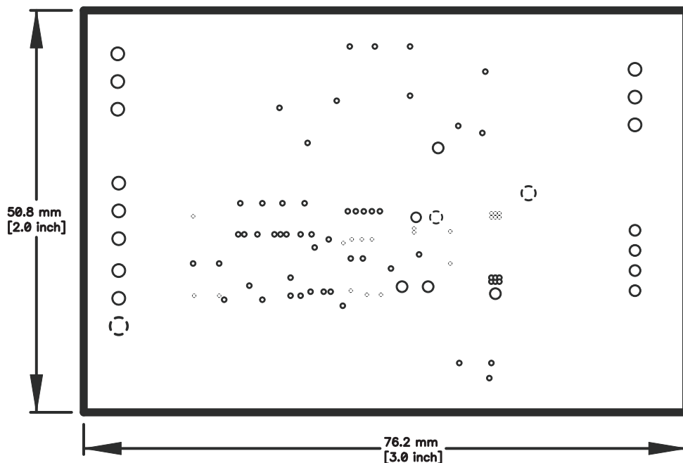
Figure 22. Internal Layer 1
