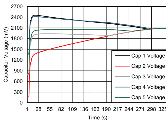
Figure 19. Voltage Convergence During Capacitor Balancing
