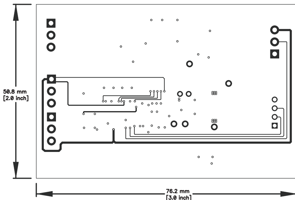
Figure 23. Internal Layer 2
